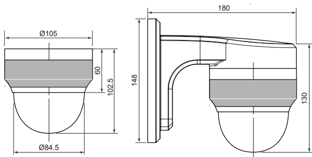
► Ceiling Type installation Dimensions ► Wall Mount Type installation Dimensions
